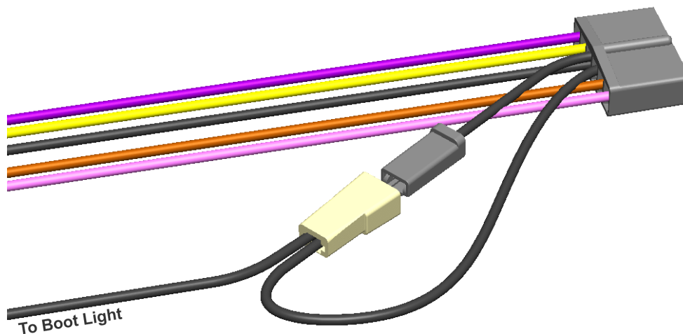
Fig 1.2 – Body Harness configured with rear compartment light
